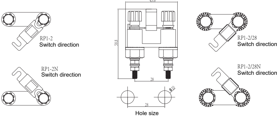
RP 1-2/28 Installation diagram
