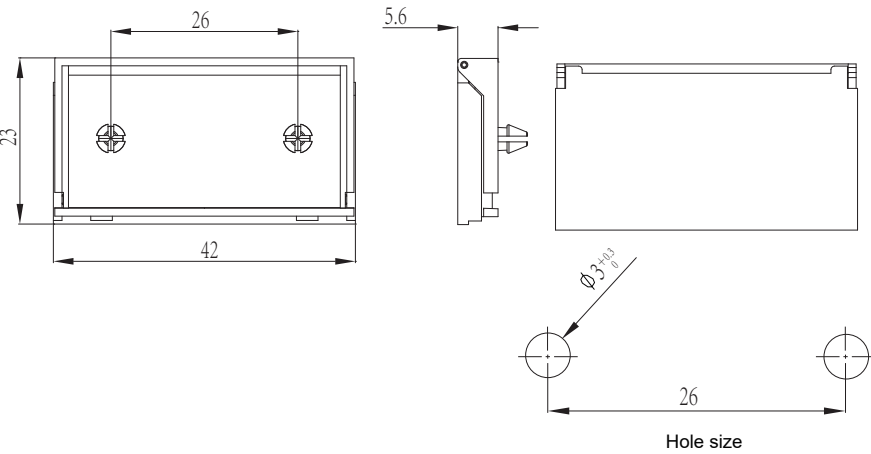
RP 1-3 Installation diagram
